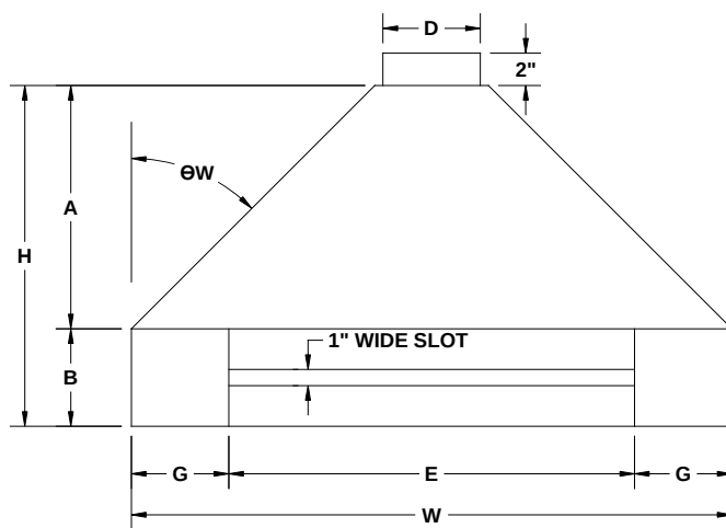
ELEVATION VIEW
