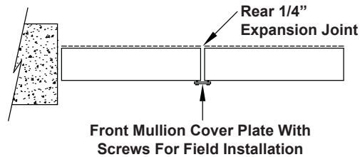
TYPICAL HORIZONTAL SECTION FOR MULTIPLE PANELS
