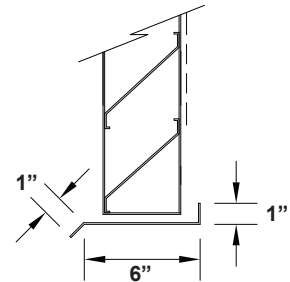
FABRICATED EXTENDED SILL
